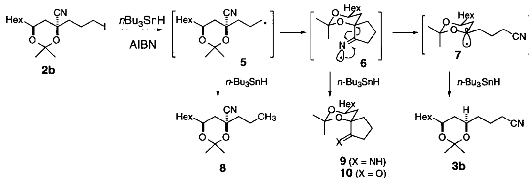
Figure 1. Possible products from the n - \text{Bu}_3\text{Sn-H} reduction of iodoalkyl nitrile 2b .
